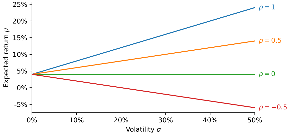
Figure 1: Expected returns from \mu = r + \lambda \rho \sigma with r = 4\% and SDF volatility \lambda = 0.4 , for four correlations between the stock and the SDF shock.
