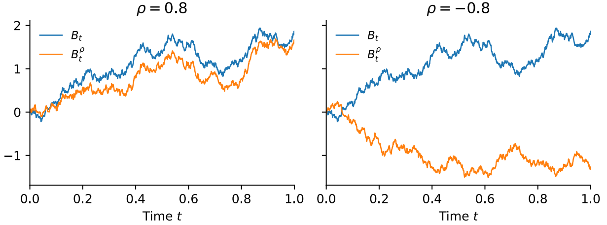
Figure 1: A Brownian path B_t and the Brownian motion B_t^\rho = \rho B_t + \sqrt{1 - \rho^2} W_t built from it and an independent path W_t . With \rho = 0.8 the two paths move together, and with \rho = -0.8 the second path mirrors the first.
