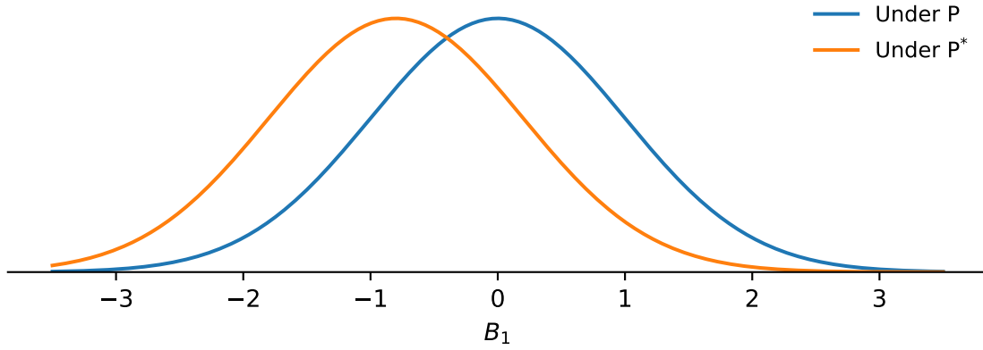
Figure 2: Density of B_1 under P and under P^* for \theta = 0.8 . Reweighting each path by Z_1 = e^{-\theta B_1 - \theta^2/2} shifts the normal density to the left by \theta and leaves its spread unchanged.
