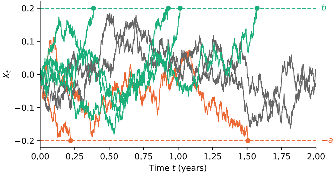
Figure 1: Eight simulated paths of X_t = \mu t + \sigma B_t with \mu = 0.05 and \sigma = 0.20 , each stopped when it reaches -a = -0.2 or b = 0.2 . By (3) a path reaches -a first with probability 0.38.
