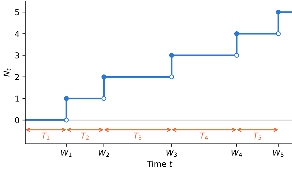
Figure 1: One simulated path of a Poisson process with rate \lambda = 1 . The arrival times W_n are marked on the time axis, and the arrows below the path show the exponential interarrival times T_n = W_n - W_{n-1} .
