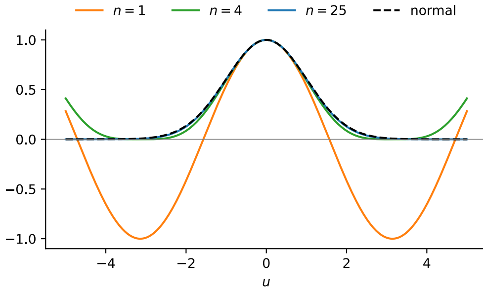
Figure 1: Characteristic function of S_n/\sqrt{n} for a fair \pm 1 coin, \cos(u/\sqrt{n})^n , against the standard normal characteristic function e^{-u^2/2} .
