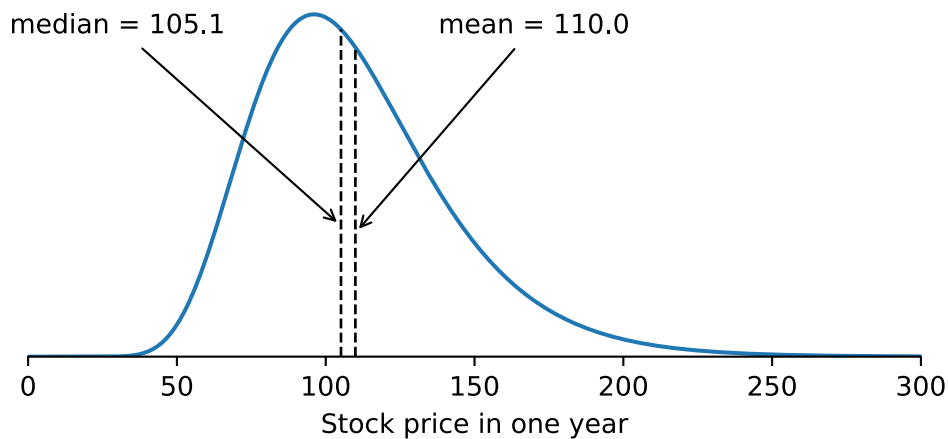
Figure 1: Density of a stock price in one year, Y = 100e^X with X \sim \mathcal{N}(0.05, 0.30^2) . The median 100e^{0.05} lies below the mean 100e^{0.05+0.045} .
