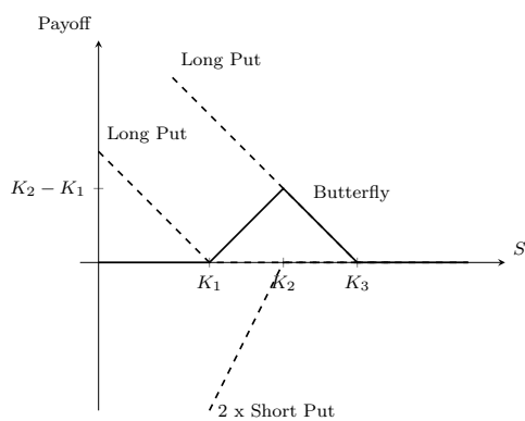
Figure 4: The butterfly can also be created using put options.
