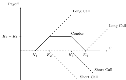
Figure 5: Payoff function of a condor strategy.
