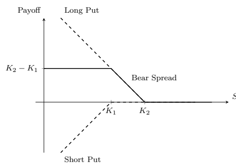
Figure 2: Payoff function of a bear spread strategy.
