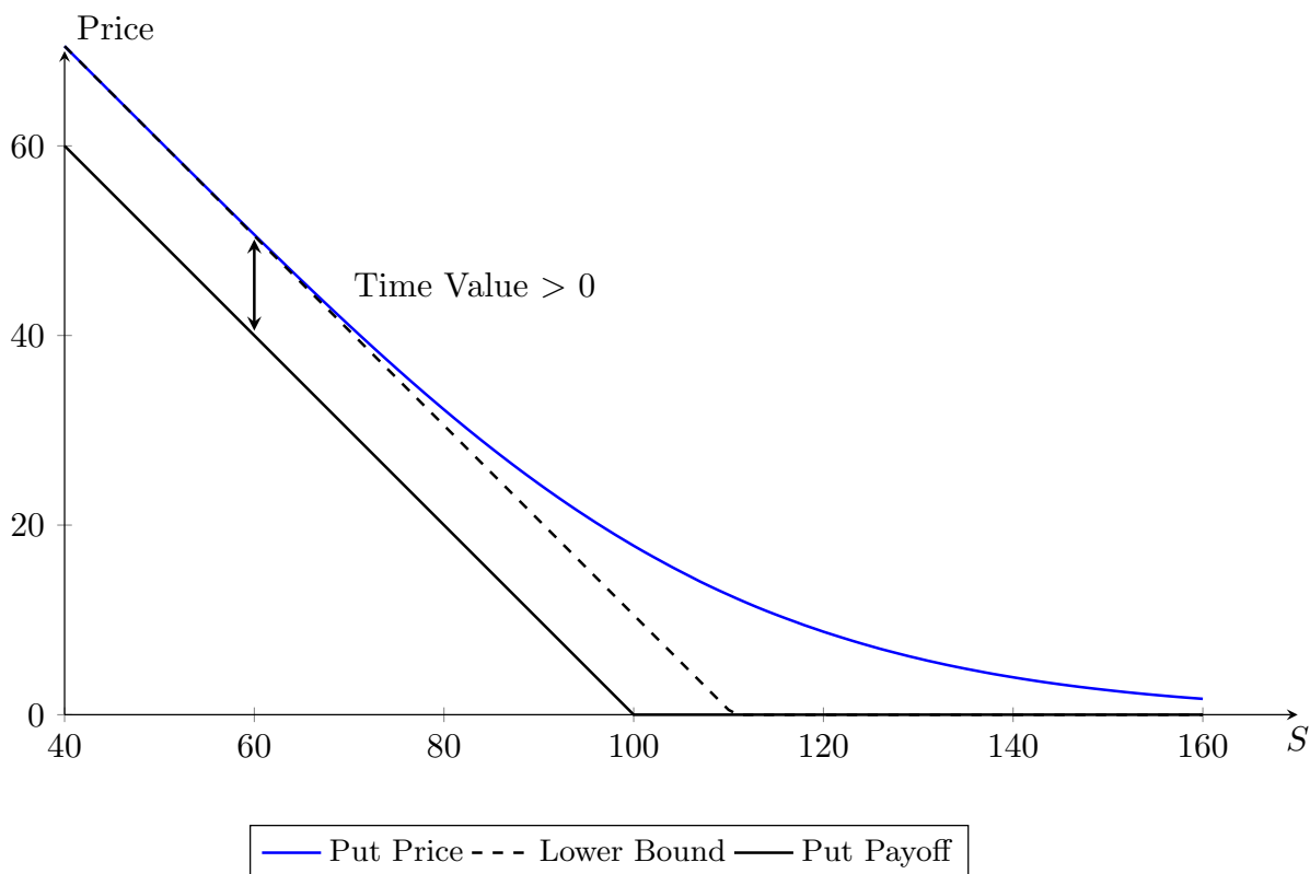
Figure 9: Hypothetical prices for a put option written on a no-dividend paying asset when the interest rate is negative.
