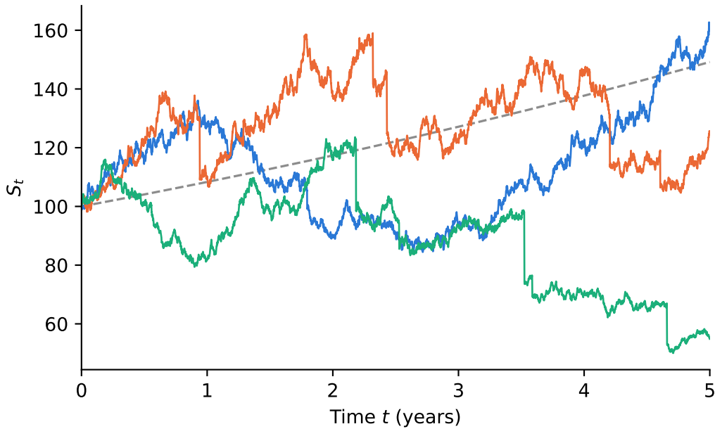
Figure 1: The figure plots three simulated paths of the Merton model with S_0 = 100 , \mu = 0.08 , \sigma = 0.15 , \lambda = 1 , m = -0.08 , and s = 0.10 over five years. The dashed line is the expected price S_0 e^{\mu t} .
