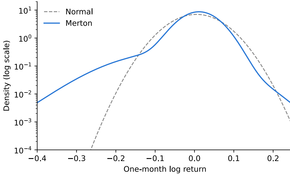
Figure 2: The figure plots the density of the one-month log return in the Merton model of Figure 1, together with a normal density with the same mean and variance, on a logarithmic scale.
