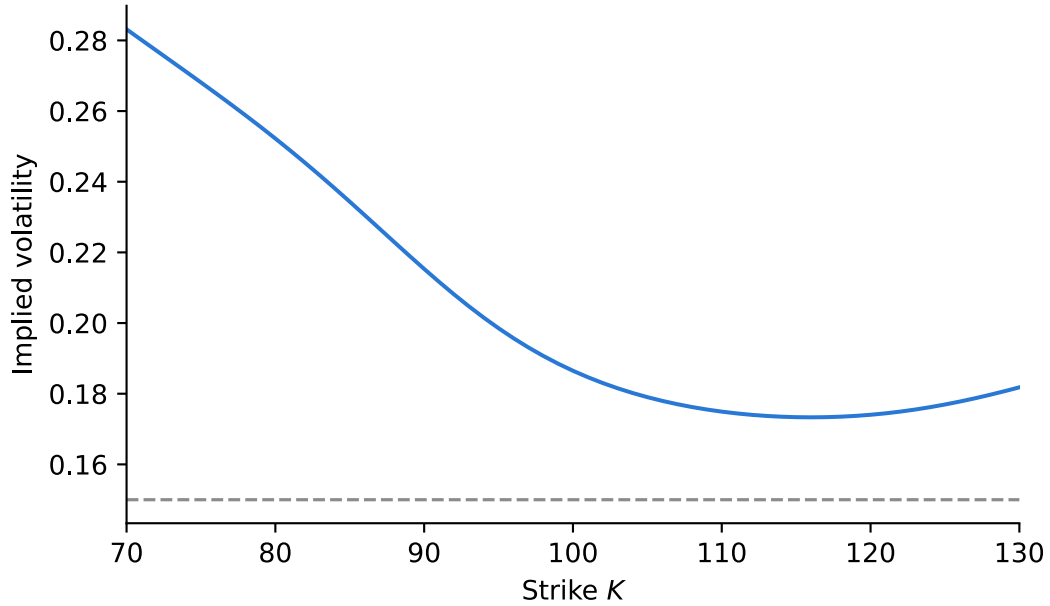
Figure 3: The figure plots the Black-Scholes implied volatility of three-month Merton call prices against the strike, with S_0 = 100 , r = 0.05 , and the jump parameters of Figure 1. The dashed line is the diffusion volatility \sigma = 0.15 .
