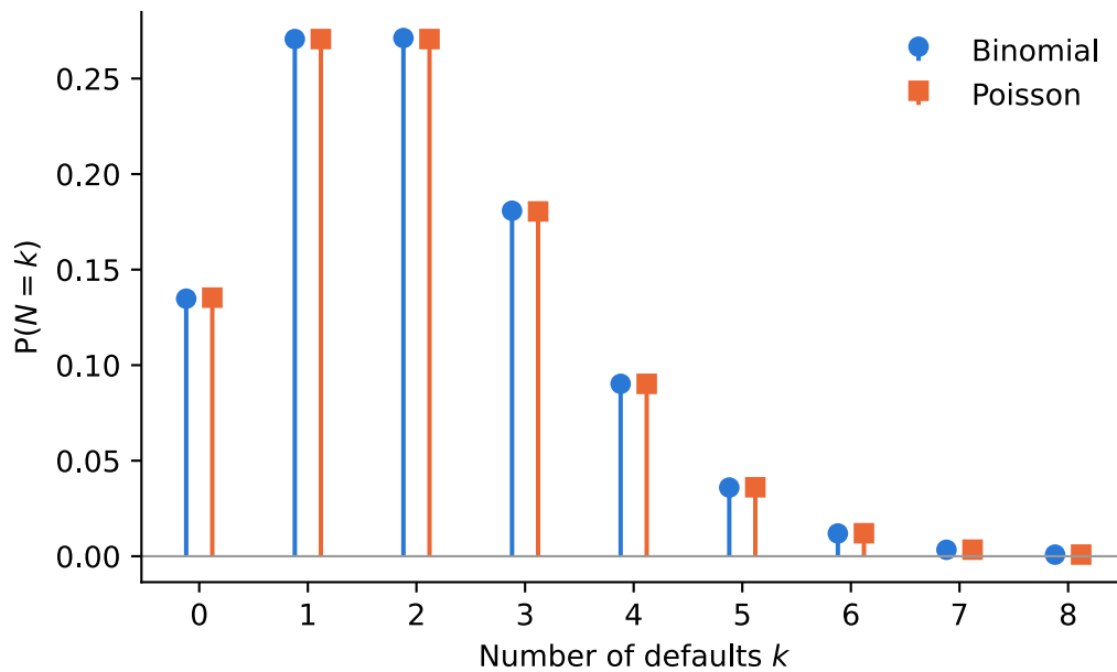
Figure 1: The figure compares the binomial distribution of the number of defaults among 500 loans, each defaulting with probability 0.004, with a Poisson distribution with the same mean \lambda = 2 .
