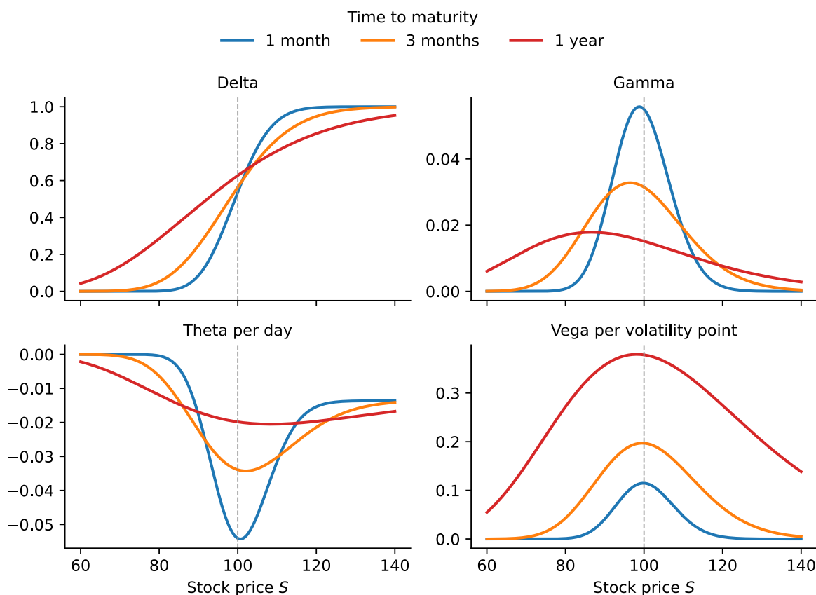
Figure 5: Delta, gamma, theta per calendar day, and vega per volatility point of a European call with K = 100 , r = 5\% , and \sigma = 25\% , against the stock price, for maturities of one month, three months, and one year. Gamma and vega are the same for the put. The dashed lines mark the strike.
