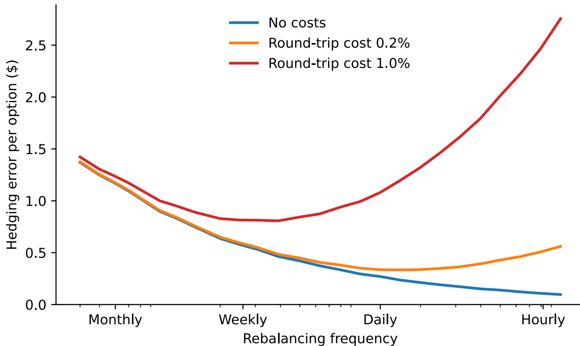
Figure 4: Root mean squared present value of the profit per option of a short call delta hedged with Black-Scholes deltas, against the number of rebalancings, on 4,000 simulated paths with constant volatility. The call has S = K = 50 , T = 0.5 , r = 5\% and \sigma = 25\% , and sells for $4.13. Each trade pays half the round-trip cost on the amount traded, so the error counts both the spread of the profit and the average cost.
