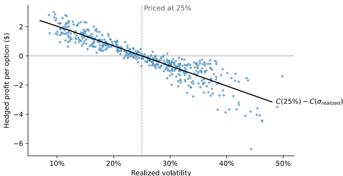
Figure 2: Profit per option of a short call hedged weekly with Black-Scholes deltas at \sigma = 25\% , against the volatility realized on each of 500 simulated paths. The call has S = K = 50 , T = 0.5 and r = 5\% . The solid line is C(25\%) - C(\sigma_{realized}) and the dashed line marks the volatility used in the price.
