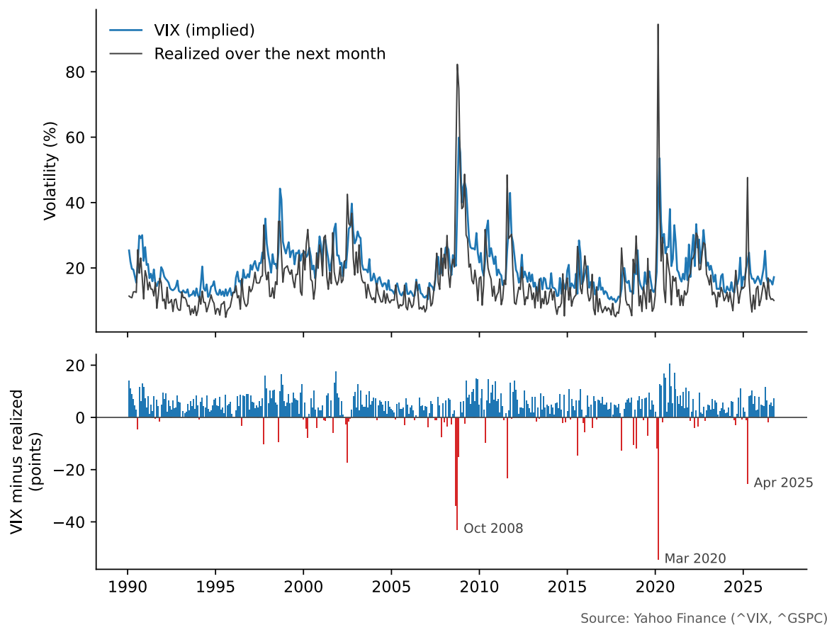
Figure 3: The top panel shows the VIX at the end of each month and the volatility of the S&P 500 realized over the following 21 trading days, both annualized. The bottom panel shows their difference, in blue when the VIX was higher and in red when realized volatility was higher. Source: Yahoo Finance.
