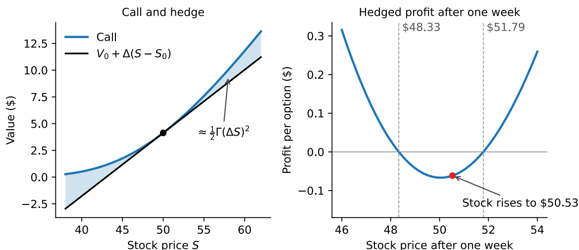
Figure 1: Left: the call of Example 1 against the stock price, with the line tangent at S_0 = 50 whose slope is \Delta = 0.591 ; the shaded gap is the value of the delta-hedged long call. Right: the profit per option of the long call, short \Delta shares and financed at r = 5\% , after one week, against the stock price at the end of the week. The dashed lines mark the breakeven prices.
