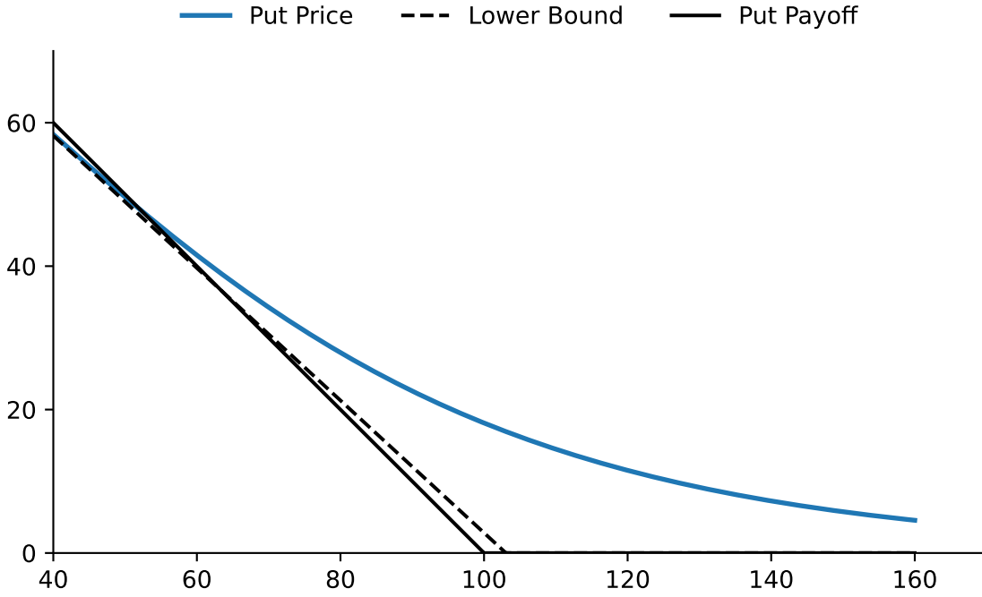
Figure 2: The figure displays the Black-Scholes put premium P(S) where r = 0.05 , \delta = 0.08 , \sigma = 0.45 , T = 1 and K = 100 . It also shows the put option payoff given by \max(K - S, 0) and the lower bound for a European put given by \max(Ke^{-rT} - Se^{-\delta T}, 0) .
