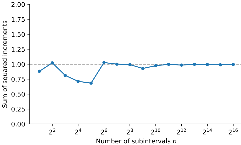
Figure 4: The figure adds up the squared increments of one simulated Brownian path on [0, 1] , using n = 2, 4, \dots, 2^{16} equal subintervals. As the subintervals shrink, the sum settles on t = 1 , the dashed line.
