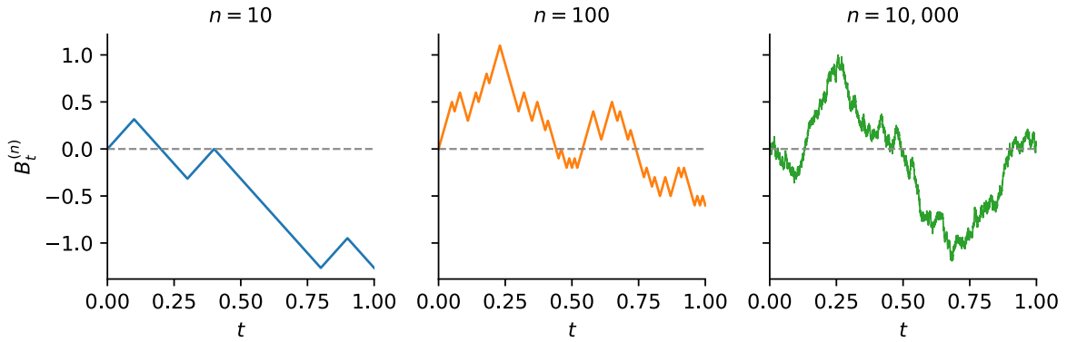
Figure 1: The figure plots one path of the scaled random walk over 0 \leq t \leq 1 with n = 10 , n = 100 , and n = 10,000 steps per unit of time. Each step moves up or down by \sqrt{\Delta t} = 1/\sqrt{n} .
