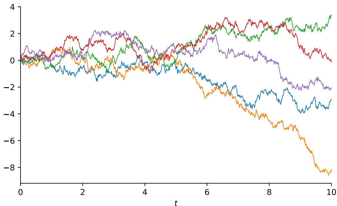
Figure 2: The figure plots simulated paths of a Brownian motion \{B_t\} for t \in [0, 10] .
