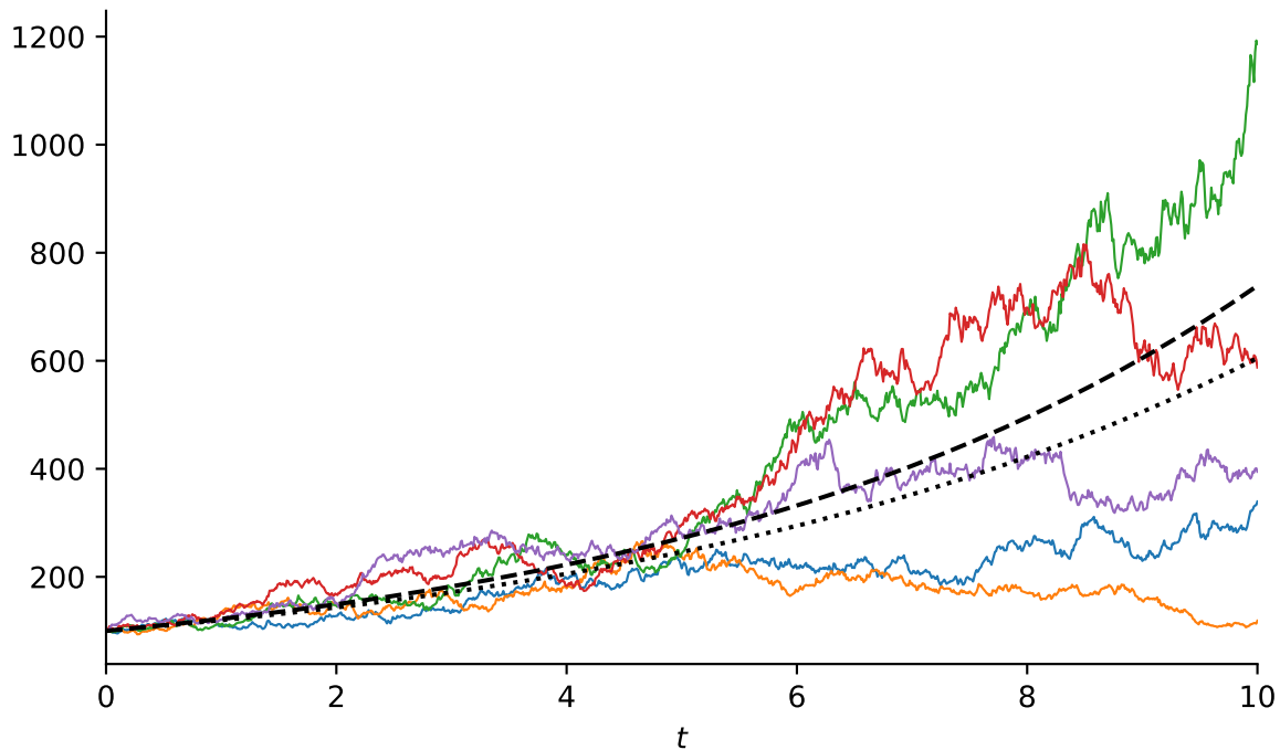
Figure 3: The figure plots simulated paths of a geometric Brownian motion \{S_t\} for t \in [0, 10] , with S_0 = 100 , \mu = 0.20 , and \sigma = 0.20 . The dashed line is the expected price \mathbb{E}(S_t) = S_0 e^{\mu t} and the dotted line is the median price S_0 e^{(\mu - \frac{1}{2}\sigma^2)t} .
