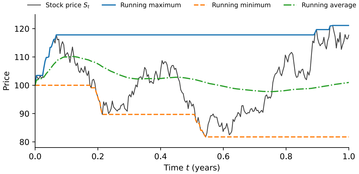
Figure 4: One simulated year of daily stock prices starting at S_0 = 100 with \sigma = 0.30 , together with the running maximum, running minimum, and running average of the path.
