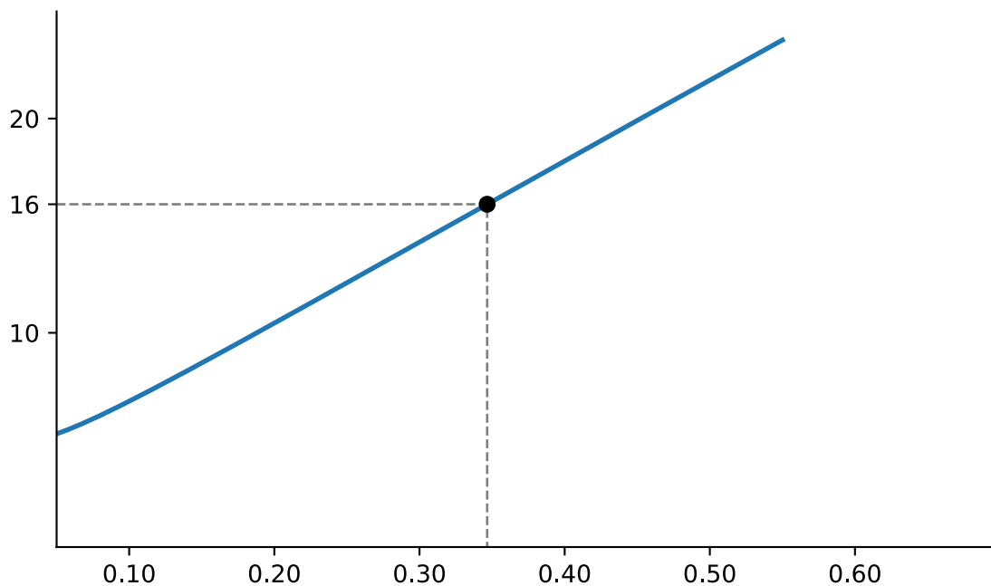
Figure 6: The figure shows the Black-Scholes call premium C(\sigma) as a function of \sigma where S = 100 , r = 0.05 , T = 1 and K = 100 . We can see that for C = \$16 the corresponding volatility is approximately 35%.
