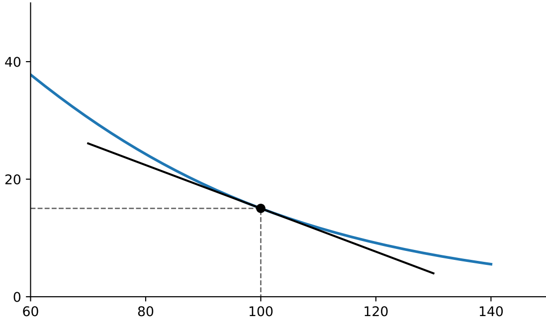
Figure 4: The figure plots the Black-Scholes put premium P(S) where r = 0.05 , \sigma = 0.45 , T = 1 and K = 100 , and shows the tangent line at S = 100 whose slope coefficient is the delta of the put given by -\Phi(-d_1) = \Phi(d_1) - 1 .
