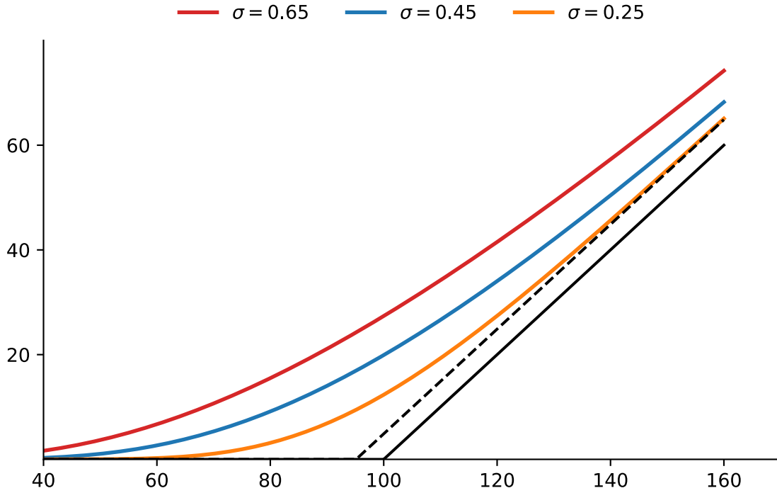
Figure 5: The figure shows the Black-Scholes call premium for different levels of volatility where r = 0.05 , T = 1 and K = 100 . The dashed line represents the lower bound for the European call and the solid black line is the call payoff at maturity.
