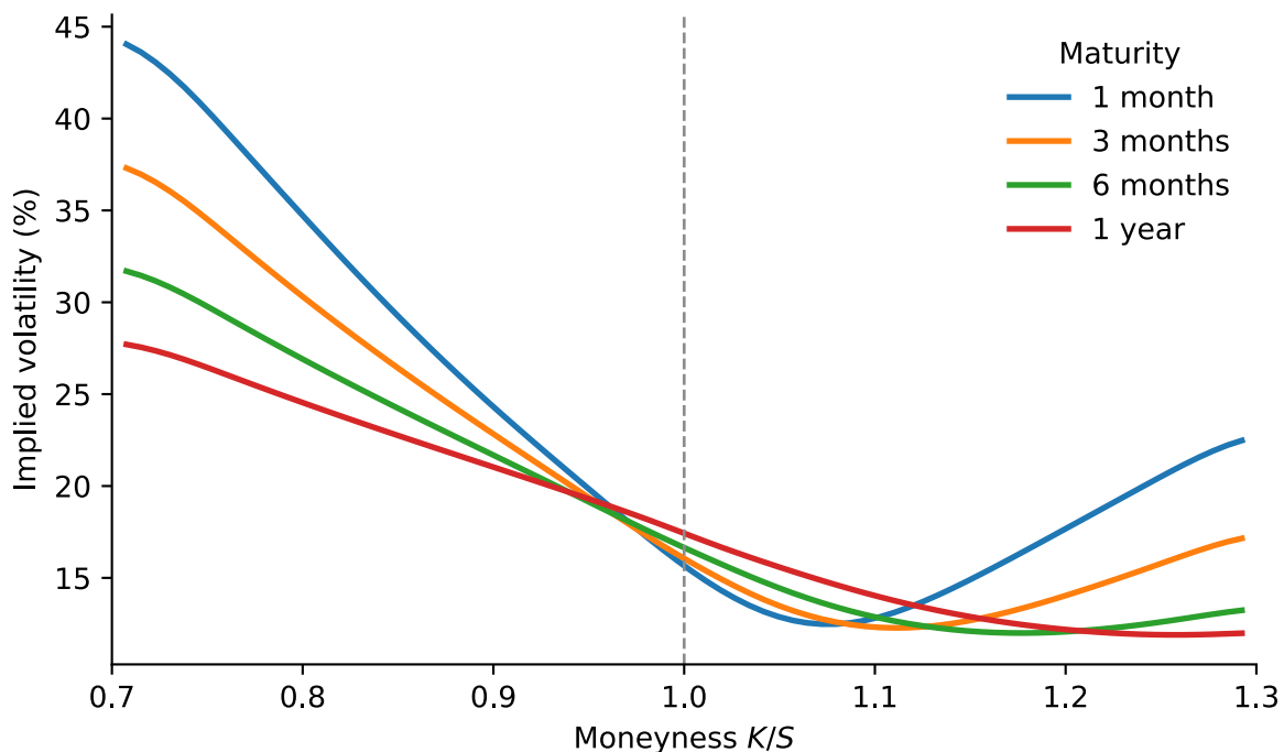
Figure 7: The figure shows the average implied volatility of S&P 500 index options against moneyness K/S for four maturities, using out-of-the-money puts for K/S < 1 and out-of-the-money calls for K/S \geq 1 . The dashed line marks at-the-money options. Source: OptionMetrics through WRDS.
