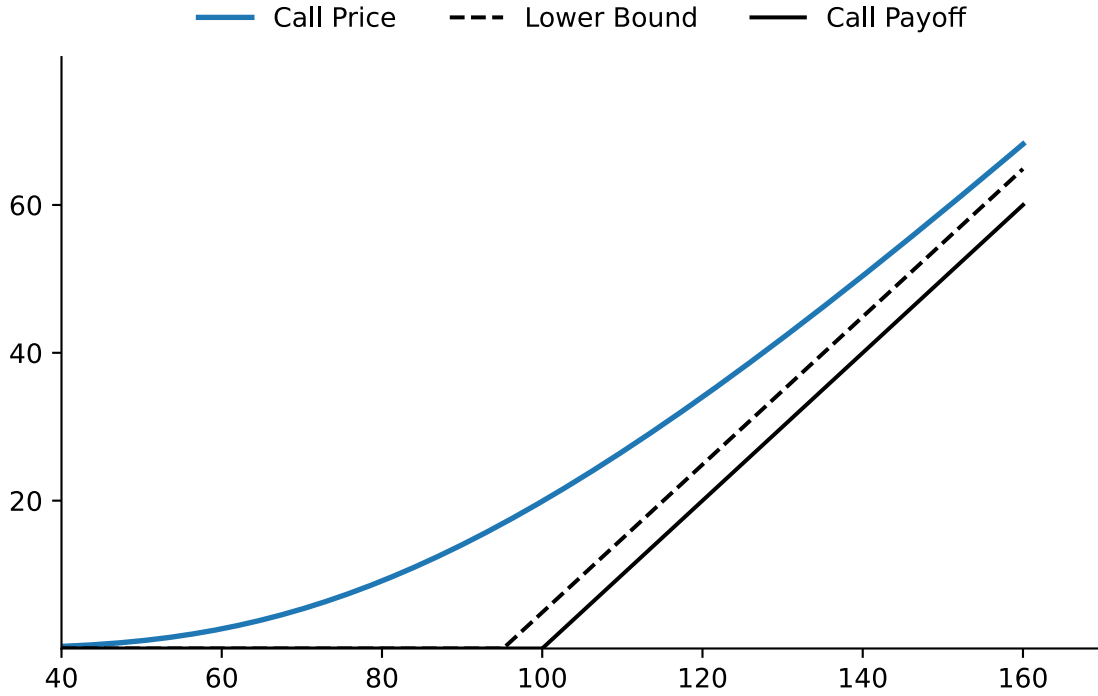
Figure 1: The figure plots the Black-Scholes call premium C(S) if r = 0.05 , \sigma = 0.45 , T = 1 and K = 100 . It also shows the call option payoff given by \max(S - K, 0) and the lower bound for a European call given by \max(S - Ke^{-rT}, 0) .
