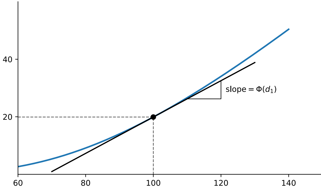
Figure 2: The figure plots the Black-Scholes call premium C(S) where r = 0.05 , \sigma = 0.45 , T = 1 and K = 100 , and shows the tangent line at S = 100 whose slope coefficient is the delta of the call given by \Phi(d_1) .
