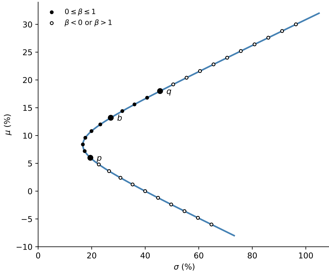
Figure 3: Spanning: combinations (1 - \beta) p + \beta q of two frontier portfolios trace out the whole MFV. Filled dots have 0 \leq \beta \leq 1 , open dots short one of the two portfolios, and b = 0.4 p + 0.6 q is labeled.
