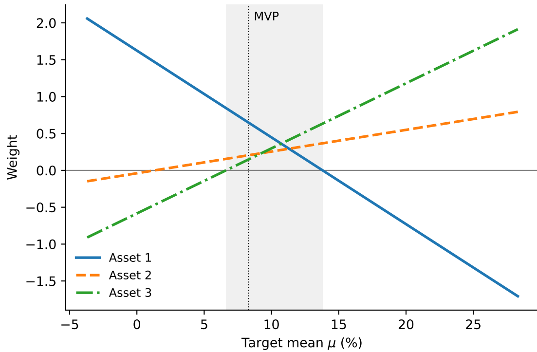
Figure 2: Frontier weights \mathbf{w} = \mathbf{a} + \mu\mathbf{b} as functions of the target mean \mu . The dotted line marks the MVP and the shaded band the targets for which all weights are positive.
