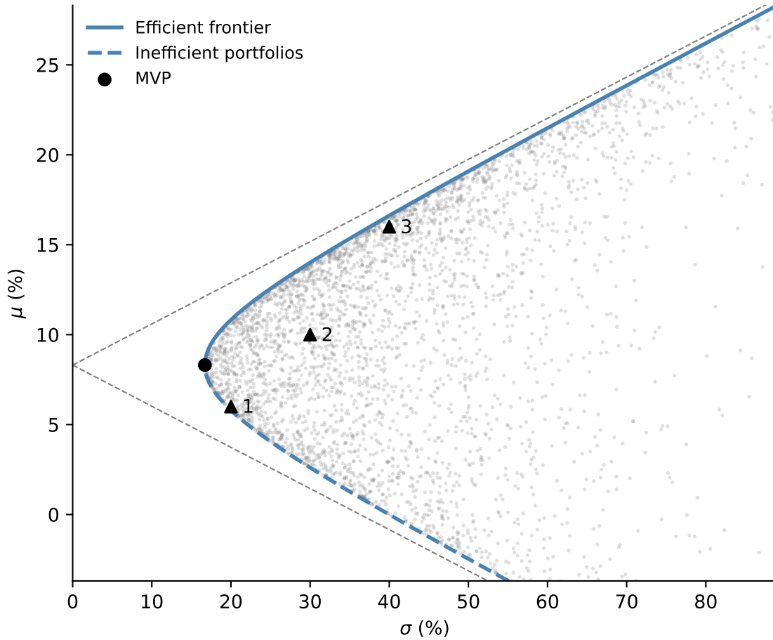
Figure 1: Minimum variance frontier for three risky assets. Gray dots are simulated portfolios obtained by perturbing the equally weighted portfolio with a random shock that sums to zero across assets. The upper branch is the efficient frontier and the dashed lines are the asymptotes.
